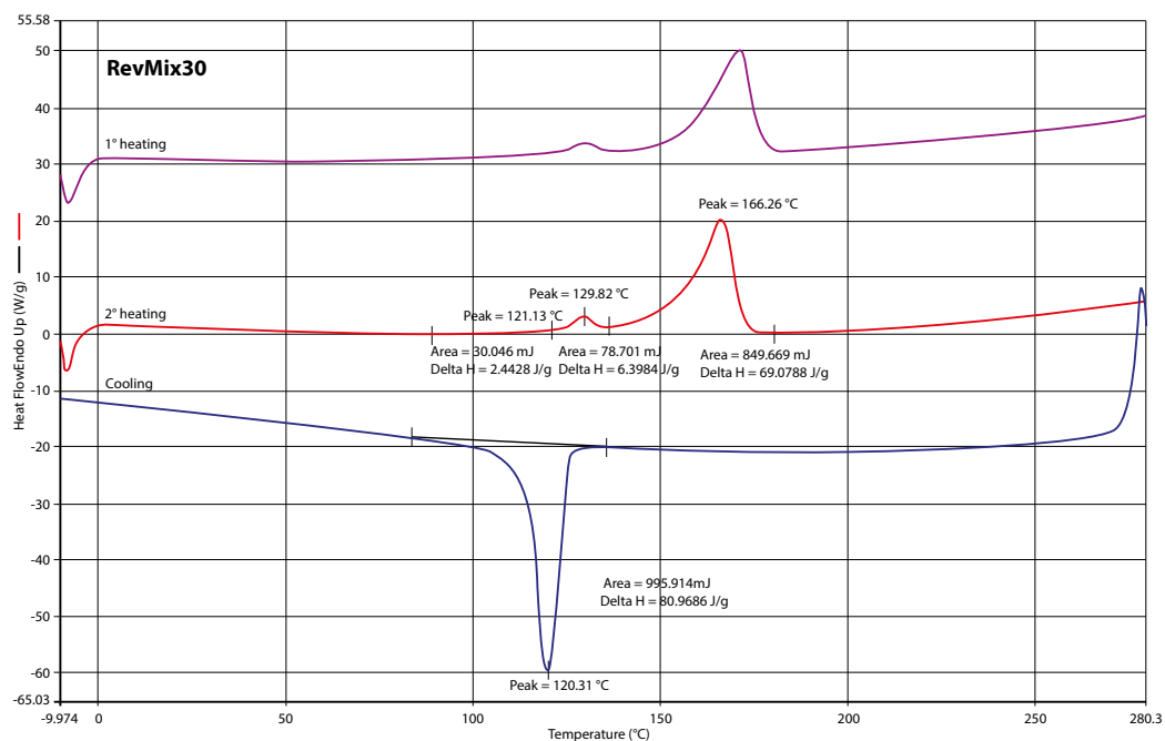
DSC RevMix 30
